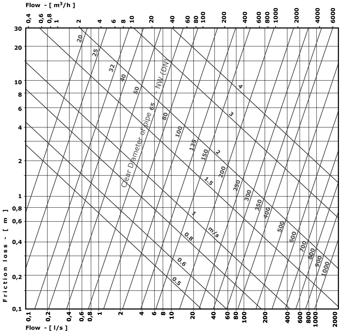
Friction loss in metres for 100m new pipeline of cast iron
