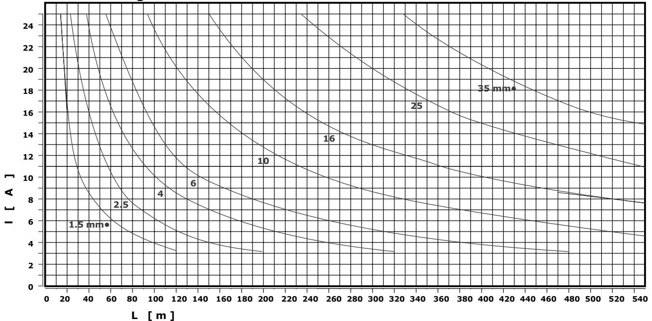
D.O.L. starting 230V multi-core cable
